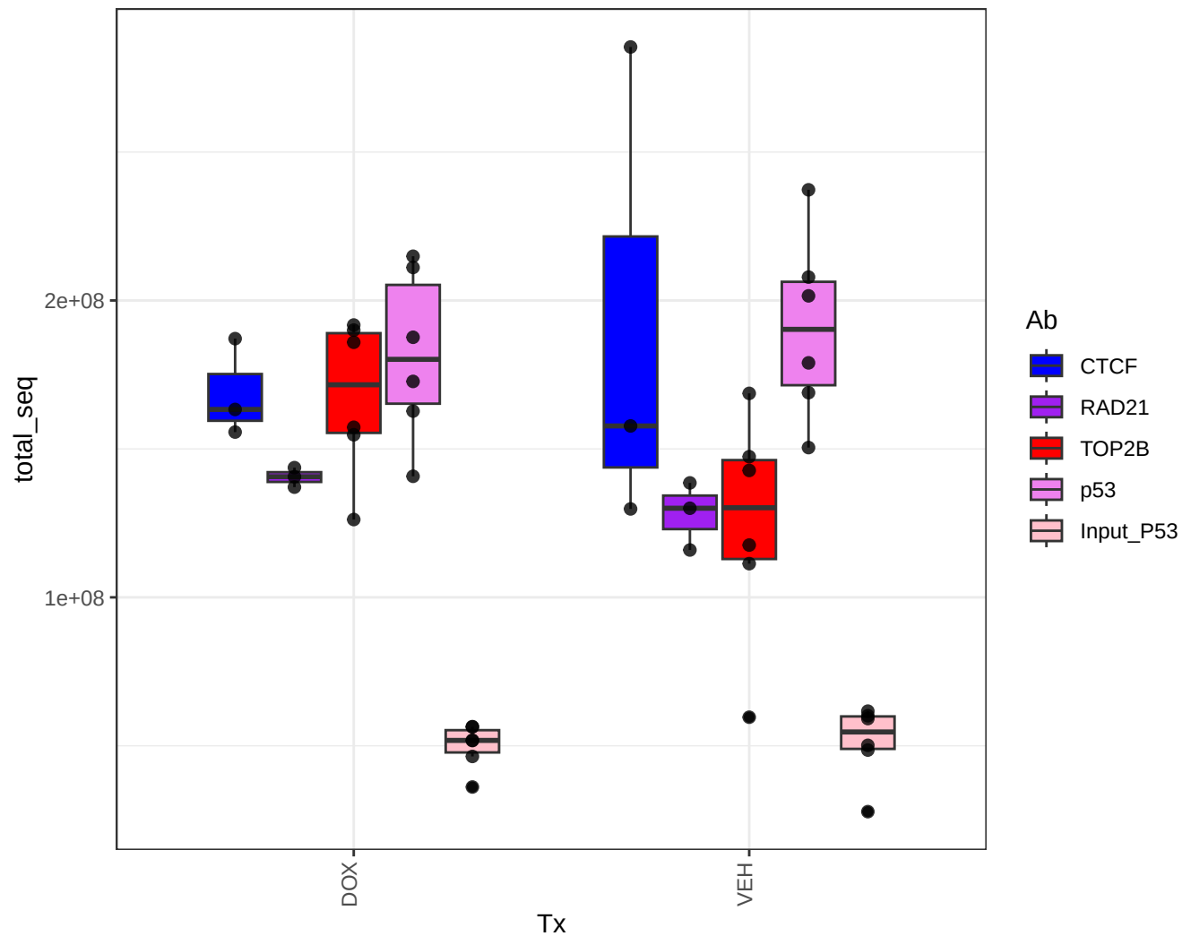
Number of sequences per sample, R1+R2 Merged Runs
